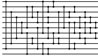
Figure 11: Evolved 11-input network with 35 comparators: [1, 10], [3, 9], [4, 8], [5, 7], [2, 6], [2, 4], [3, 5], [7, 11], [8, 9], [6, 10], [1, 7], [2, 3], [9, 11], [10, 11], [1, 2], [6, 8], [4, 5], [7, 9], [3, 7], [2, 6], [8, 9], [5, 10], [3, 4], [9, 10], [2, 3], [5, 7], [4, 6], [7, 8], [8, 9], [3, 4], [5, 7], [6, 7], [4, 5], [7, 8], [5, 6].
