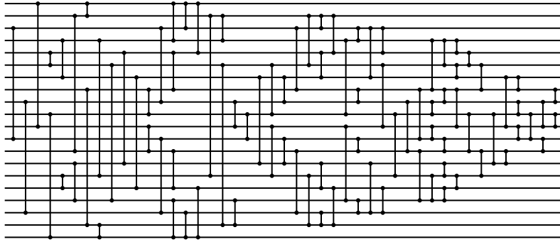
Figure 20: Evolved 20-input network with 92 comparators: [3, 12], [9, 18], [1, 11], [10, 20], [5, 6], [15, 16], [4, 7], [14, 17], [2, 13], [8, 19], [4, 15], [6, 17], [1, 2], [19, 20], [5, 14], [7, 16], [8, 10], [11, 13], [3, 9], [12, 18], [5, 8], [13, 16], [1, 4], [17, 20], [1, 3], [18, 20], [1, 5], [16, 20], [2, 15], [6, 19], [9, 11], [10, 12], [7, 14], [6, 10], [11, 15], [2, 4], [17, 19], [7, 9], [12, 14], [3, 8], [13, 18], [2, 6], [2, 3], [15, 19], [5, 7], [14, 16], [18, 19], [16, 19], [2, 5], [4, 10], [11, 17], [3, 4], [17, 18], [14, 18], [3, 7], [16, 18], [3, 5], [8, 9], [12, 13], [6, 11], [10, 15], [9, 13], [8, 12], [4, 8], [13, 17], [4, 6], [15, 17], [16, 17], [4, 5], [6, 7], [14, 15], [15, 16], [5, 6], [11, 12], [9, 10], [12, 13], [8, 9], [8, 11], [10, 13], [6, 8], [13, 15], [10, 14], [7, 11], [7, 8], [11, 12], [13, 14], [9, 10], [10, 12], [12, 13], [9, 11], [8, 9], [10, 11].
