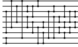
Figure 9: Evolved 9-input network with 25 comparators: [3, 7], [1, 6], [2, 5], [8, 9], [1, 8], [2, 3], [4, 6], [5, 7], [6, 9], [2, 4], [7, 9], [1, 2], [5, 6], [3, 8], [4, 8], [4, 5], [6, 7], [2, 3], [2, 4], [7, 8], [5, 6], [3, 5], [6, 7], [3, 4], [5, 6].
