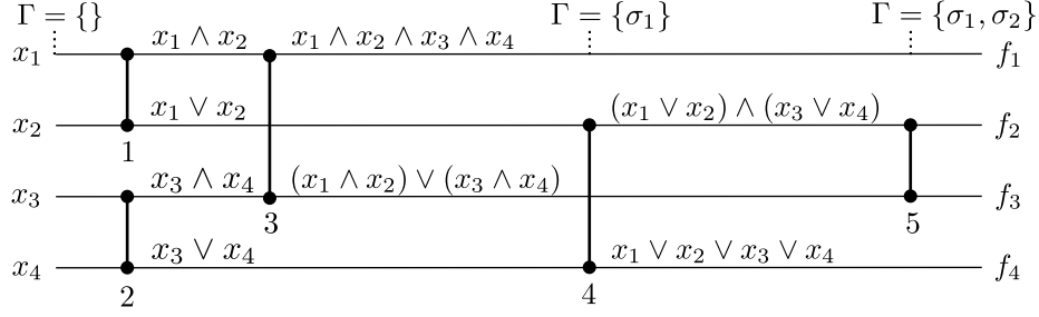
Figure 6: Subgoals for constructing a minimal 4-input sorting network. The final goal is to produce the symmetry \Gamma = \{\sigma_1, \sigma_2\} by computing all four output functions f_i while utilizing the minimum number of comparators. This goal can be decomposed into a sequence of subgoals specified as subgroups of the final symmetry group \langle \Gamma \rangle . At any stage in the construction, the next subgoal is the subgroup that can be produced by adding the fewest number of comparators. Initially, the network does not have any symmetries, i.e. \Gamma = \{\} . The dual functions f_1 and f_4 are the easiest to compute, having fewer variable combinations and therefore requiring fewer comparators than f_2 and f_3 . Hence the first subgoal is to produce the symmetry \Gamma = \{\sigma_1\} . Notice that comparators 1 and 2 compute parts of both f_1 and f_4 to achieve this subgoal with the minimum number of comparators. The second subgoal is to produce the symmetry \Gamma = \{\sigma_1, \sigma_2\} by computing the functions f_2 and f_3 . Adding comparator 5 completes this subgoal since comparators 3 and 4 have already computed f_2 and f_3 partially. Optimizing the number of comparators required to reach each subgoal separately in this way makes it possible to scale the approach to networks with more inputs.
