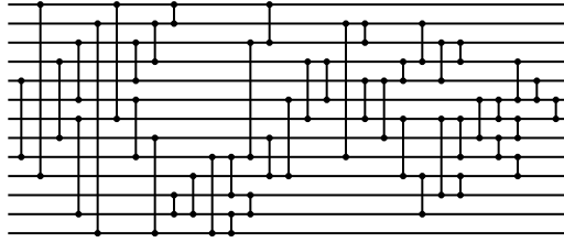
Figure 13: Evolved 13-input network with 45 comparators: [5, 9], [1, 10], [4, 8], [3, 6], [7, 12], [2, 13], [1, 7], [3, 5], [6, 9], [8, 13], [2, 4], [11, 12], [10, 12], [1, 2], [9, 13], [9, 11], [3, 9], [12, 13], [1, 3], [8, 10], [6, 10], [4, 7], [4, 6], [2, 9], [5, 7], [5, 8], [11, 12], [7, 10], [4, 5], [2, 3], [10, 12], [2, 4], [7, 11], [3, 5], [3, 4], [10, 11], [7, 9], [6, 8], [6, 7], [8, 9], [4, 6], [9, 10], [5, 6], [7, 8], [6, 7].
