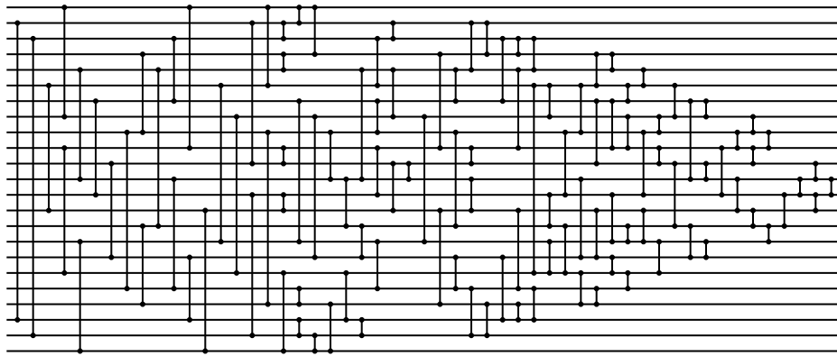
Figure 23: Evolved 23-input network with 118 comparators: [2, 21], [3, 22], [6, 14], [10, 18], [1, 8], [16, 23], [5, 12], [7, 13], [11, 17], [9, 19], [15, 20], [4, 9], [5, 15], [12, 19], [3, 7], [17, 21], [1, 10], [14, 23], [6, 16], [8, 18], [2, 11], [13, 22], [9, 20], [18, 23], [1, 6], [21, 22], [2, 3], [19, 20], [4, 5], [22, 23], [1, 2], [20, 23], [1, 4], [13, 14], [10, 11], [7, 16], [8, 17], [9, 12], [12, 15], [5, 12], [7, 9], [15, 17], [18, 21], [3, 6], [10, 13], [11, 14], [16, 19], [11, 12], [5, 8], [21, 22], [2, 3], [8, 16], [4, 10], [14, 20], [17, 19], [9, 15], [5, 7], [19, 22], [2, 5], [20, 22], [2, 4], [10, 11], [12, 14], [3, 7], [17, 21], [5, 10], [14, 19], [20, 21], [3, 4], [19, 21], [3, 5], [6, 18], [13, 15], [9, 13], [6, 8], [16, 18], [6, 9], [15, 18], [4, 6], [18, 20], [4, 5], [19, 20], [7, 11], [12, 17], [14, 17], [7, 10], [17, 18], [6, 7], [5, 6], [8, 10], [18, 19], [13, 16], [15, 16], [9, 13], [8, 9], [14, 16], [16, 18], [6, 8], [10, 11], [11, 15], [7, 12], [15, 17], [16, 17], [7, 8], [11, 12], [10, 13], [12, 14], [14, 15], [9, 10], [8, 9], [15, 16], [10, 11], [9, 10], [13, 15], [12, 13], [13, 14], [11, 12], [12, 13].
