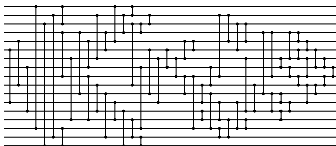
Figure 17: Evolved 17-input network with 71 comparators: [6, 12], [5, 10], [8, 13], [1, 15], [3, 17], [2, 16], [4, 9], [7, 14], [4, 11], [9, 14], [5, 8], [10, 13], [1, 3], [15, 17], [2, 7], [11, 16], [4, 6], [12, 14], [1, 5], [13, 17], [2, 4], [14, 16], [1, 2], [16, 17], [3, 10], [8, 15], [6, 11], [7, 12], [6, 8], [7, 9], [9, 11], [3, 4], [9, 15], [10, 12], [13, 14], [5, 7], [11, 15], [5, 6], [8, 10], [12, 14], [2, 3], [15, 16], [2, 9], [14, 16], [2, 5], [3, 6], [12, 15], [14, 15], [3, 5], [7, 13], [10, 13], [4, 11], [4, 9], [7, 8], [11, 13], [4, 7], [4, 5], [13, 14], [11, 12], [6, 7], [12, 13], [5, 6], [8, 9], [9, 10], [7, 9], [10, 12], [6, 8], [7, 8], [10, 11], [9, 10], [8, 9].
