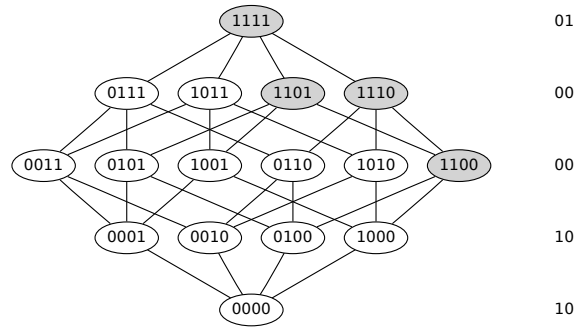
Figure 8: State representation of the function x_1 \wedge x_2 utilized in the EDA. The state (shown on the right) is a bit-string with two bits for each level of the Boolean lattice. The first bit is 1 only if the value of the function for all nodes in that level is 0 and the second bit is 1 only if its value for all nodes in that level is 1. This condensed representation of the function is based on the information utilized by the symmetry-building greedy algorithm and it is therefore useful for constructing minimal-size sorting networks.
