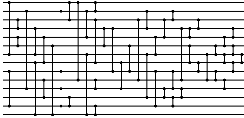
Figure 14: Evolved 14-input network with 51 comparators: [1, 7], [3, 4], [9, 13], [5, 6], [2, 11], [8, 14], [10, 12], [4, 7], [5, 8], [6, 14], [2, 9], [11, 13], [1, 3], [12, 13], [1, 10], [2, 5], [7, 14], [13, 14], [1, 2], [3, 8], [4, 6], [10, 11], [4, 9], [8, 11], [6, 9], [3, 10], [7, 12], [5, 7], [9, 13], [2, 4], [11, 12], [3, 5], [12, 13], [2, 3], [9, 11], [4, 10], [4, 5], [3, 4], [11, 12], [6, 8], [8, 9], [7, 10], [6, 7], [5, 6], [9, 10], [7, 8], [10, 11], [4, 5], [6, 7], [8, 9], [7, 8].
