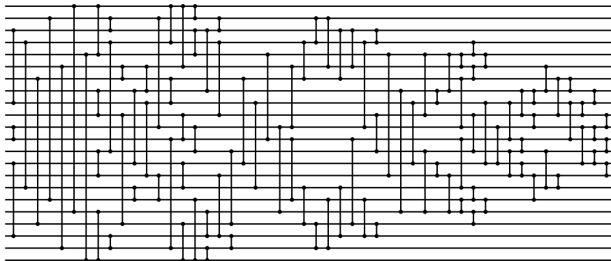
Figure 22: Evolved 22-input network with 108 comparators: [11, 12], [3, 9], [14, 20], [4, 16], [7, 19], [2, 17], [6, 21], [1, 18], [5, 22], [8, 10], [13, 15], [1, 5], [18, 22], [4, 13], [10, 19], [2, 3], [20, 21], [8, 14], [9, 15], [6, 7], [16, 17], [6, 8], [15, 17], [2, 11], [12, 21], [1, 4], [19, 22], [1, 6], [17, 22], [1, 2], [21, 22], [7, 9], [14, 16], [3, 5], [18, 20], [10, 12], [11, 13], [3, 8], [15, 20], [4, 10], [13, 19], [7, 14], [9, 16], [5, 12], [11, 18], [6, 11], [12, 17], [4, 7], [16, 19], [2, 3], [20, 21], [2, 4], [19, 21], [2, 6], [17, 21], [3, 7], [16, 20], [12, 19], [3, 6], [17, 20], [4, 11], [3, 4], [19, 20], [10, 13], [5, 15], [8, 18], [9, 14], [13, 18], [5, 10], [14, 15], [8, 9], [5, 8], [15, 18], [5, 6], [17, 18], [18, 19], [4, 5], [7, 11], [12, 16], [6, 7], [16, 17], [5, 6], [17, 18], [10, 13], [9, 14], [11, 14], [9, 12], [8, 10], [13, 15], [8, 9], [14, 15], [15, 17], [6, 8], [10, 11], [12, 13], [7, 10], [13, 16], [15, 16], [7, 8], [9, 12], [11, 14], [9, 10], [13, 14], [8, 9], [14, 15], [11, 12], [12, 13], [10, 11].
