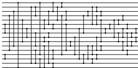
Figure 16: Evolved 16-input network with 60 comparators: [13, 14], [6, 8], [4, 12], [3, 11], [1, 16], [5, 10], [7, 9], [2, 15], [12, 15], [2, 4], [8, 11], [1, 13], [5, 7], [3, 6], [9, 10], [14, 16], [11, 16], [1, 3], [10, 15], [2, 5], [1, 2], [15, 16], [6, 7], [8, 9], [12, 14], [4, 13], [6, 12], [10, 11], [9, 13], [3, 5], [7, 14], [4, 8], [3, 4], [13, 15], [11, 14], [2, 6], [14, 15], [2, 3], [4, 6], [11, 13], [13, 14], [3, 4], [9, 12], [5, 10], [11, 12], [7, 8], [6, 7], [5, 9], [8, 10], [5, 6], [10, 12], [12, 13], [4, 5], [7, 9], [8, 11], [10, 11], [6, 7], [8, 9], [9, 10], [7, 8].
