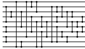
Figure 10: Evolved 10-input network with 29 comparators: [2, 5], [8, 9], [3, 4], [6, 7], [1, 10], [3, 6], [1, 8], [9, 10], [4, 7], [5, 10], [1, 2], [1, 3], [7, 10], [4, 6], [5, 8], [2, 9], [4, 5], [6, 9], [7, 8], [2, 3], [8, 9], [2, 4], [3, 6], [5, 7], [3, 4], [7, 8], [5, 6], [4, 5], [6, 7].
