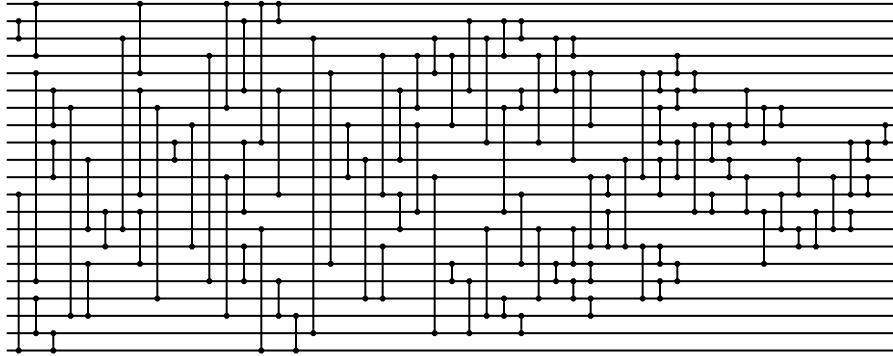
Figure 21: Evolved 21-input network with 103 comparators: [12, 21], [2, 3], [5, 17], [9, 11], [18, 20], [6, 8], [7, 19], [10, 14], [13, 15], [1, 4], [3, 14], [1, 5], [20, 21], [16, 19], [6, 12], [13, 16], [7, 18], [9, 10], [8, 15], [4, 17], [11, 19], [9, 13], [15, 17], [1, 7], [14, 21], [2, 6], [1, 9], [17, 19], [19, 21], [1, 2], [6, 12], [3, 20], [5, 16], [8, 11], [10, 18], [4, 12], [6, 10], [12, 14], [8, 13], [15, 18], [4, 7], [11, 20], [3, 5], [16, 17], [4, 8], [2, 6], [17, 20], [3, 9], [14, 19], [2, 4], [18, 19], [19, 20], [2, 3], [7, 13], [12, 16], [6, 7], [14, 18], [16, 17], [4, 9], [17, 18], [3, 6], [18, 19], [3, 4], [14, 16], [11, 15], [5, 10], [5, 8], [11, 12], [13, 15], [10, 15], [5, 11], [5, 6], [16, 17], [15, 18], [17, 18], [4, 5], [7, 9], [10, 12], [6, 7], [9, 11], [15, 16], [5, 6], [16, 17], [8, 13], [12, 13], [8, 10], [10, 11], [11, 13], [8, 9], [6, 8], [13, 16], [12, 14], [7, 9], [14, 15], [7, 8], [13, 15], [10, 12], [11, 14], [9, 12], [9, 10], [8, 9], [11, 12], [13, 14].
