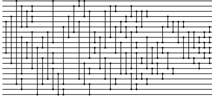
Figure 19: Evolved 19-input network with 86 comparators: [5, 11], [4, 13], [1, 17], [8, 15], [9, 12], [7, 14], [16, 18], [2, 6], [10, 19], [3, 6], [12, 17], [8, 10], [2, 3], [7, 16], [11, 13], [4, 5], [14, 18], [1, 9], [15, 19], [6, 17], [4, 8], [18, 19], [2, 7], [5, 16], [1, 2], [13, 17], [1, 4], [17, 19], [3, 12], [10, 11], [14, 15], [7, 9], [8, 14], [3, 10], [12, 16], [2, 8], [6, 11], [13, 18], [9, 15], [5, 7], [11, 15], [4, 5], [16, 17], [2, 3], [15, 18], [2, 4], [17, 18], [6, 8], [7, 14], [6, 7], [11, 16], [3, 5], [15, 16], [3, 6], [12, 13], [16, 17], [3, 4], [9, 10], [8, 14], [10, 13], [9, 12], [10, 11], [14, 15], [6, 9], [13, 15], [15, 16], [4, 6], [5, 7], [11, 14], [5, 9], [5, 6], [14, 15], [8, 12], [7, 12], [7, 10], [8, 9], [12, 13], [7, 8], [13, 14], [6, 7], [10, 11], [11, 12], [12, 13], [9, 10], [8, 9], [10, 11].
