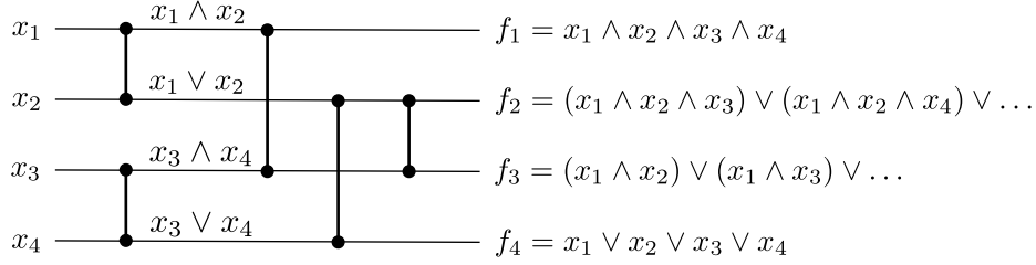
Figure 3: Boolean output functions of a 4-input sorting network. The zero-one principle can be utilized to represent the inputs of the network as Boolean variables. Each comparator produces the conjunction of its inputs on its upper line and their disjunction on its lower line. As a result, the functions at the outputs of the network are compositions of conjunctions and disjunctions of the input variables, i.e. they are monotone Boolean functions. In particular, the output function f_i at line i is the disjunction of all conjunctive terms with exactly n + 1 - i variables. Therefore, a sorting network is a sequence of comparators that compute all its output functions from its input variables. This representation makes it possible to express network symmetry, which turns out to be useful in constructing minimal networks.
