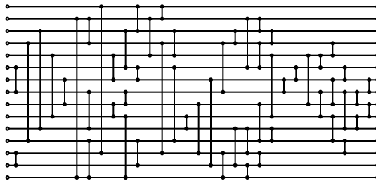
Figure 15: Evolved 15-input network with 56 comparators: [13, 14], [6, 8], [4, 12], [3, 11], [5, 10], [7, 9], [2, 15], [12, 15], [2, 4], [8, 11], [1, 13], [5, 7], [3, 6], [9, 10], [1, 3], [10, 15], [2, 5], [1, 2], [6, 7], [8, 9], [12, 14], [4, 13], [6, 12], [10, 11], [9, 13], [3, 5], [7, 14], [4, 8], [3, 4], [13, 15], [11, 14], [2, 6], [14, 15], [2, 3], [4, 6], [11, 13], [13, 14], [3, 4], [9, 12], [5, 10], [11, 12], [7, 8], [6, 7], [5, 9], [8, 10], [5, 6], [10, 12], [12, 13], [4, 5], [7, 9], [8, 11], [10, 11], [6, 7], [8, 9], [9, 10], [7, 8].
