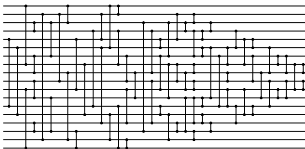
Figure 18: Evolved 18-input network with 78 comparators: [5, 13], [6, 14], [1, 8], [11, 18], [3, 4], [15, 16], [7, 9], [10, 12], [2, 17], [3, 7], [12, 16], [2, 10], [9, 17], [5, 11], [8, 14], [4, 13], [6, 15], [1, 3], [16, 18], [2, 5], [14, 17], [1, 6], [13, 18], [1, 2], [17, 18], [4, 8], [11, 15], [7, 10], [9, 12], [3, 16], [4, 9], [10, 15], [5, 6], [13, 14], [7, 11], [3, 7], [8, 12], [2, 5], [14, 17], [15, 16], [3, 4], [12, 16], [16, 17], [2, 3], [12, 15], [4, 7], [14, 15], [4, 5], [15, 16], [3, 4], [6, 7], [12, 13], [8, 10], [9, 11], [10, 11], [8, 9], [6, 12], [7, 13], [11, 13], [6, 8], [13, 15], [4, 6], [11, 14], [5, 8], [13, 14], [5, 6], [9, 10], [7, 10], [9, 12], [10, 13], [6, 9], [7, 8], [11, 12], [7, 9], [10, 12], [8, 11], [10, 11], [8, 9].
