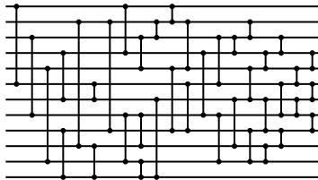
Figure 12: Evolved 12-input network with 39 comparators: [1, 6], [3, 8], [5, 11], [4, 7], [9, 12], [2, 10], [6, 7], [2, 9], [1, 4], [3, 5], [10, 12], [8, 11], [8, 10], [11, 12], [2, 3], [7, 12], [1, 2], [5, 9], [6, 9], [2, 5], [4, 8], [3, 6], [8, 11], [7, 10], [3, 4], [5, 7], [9, 11], [2, 3], [10, 11], [7, 9], [4, 5], [9, 10], [3, 4], [6, 8], [5, 6], [7, 8], [8, 9], [6, 7], [4, 5].
