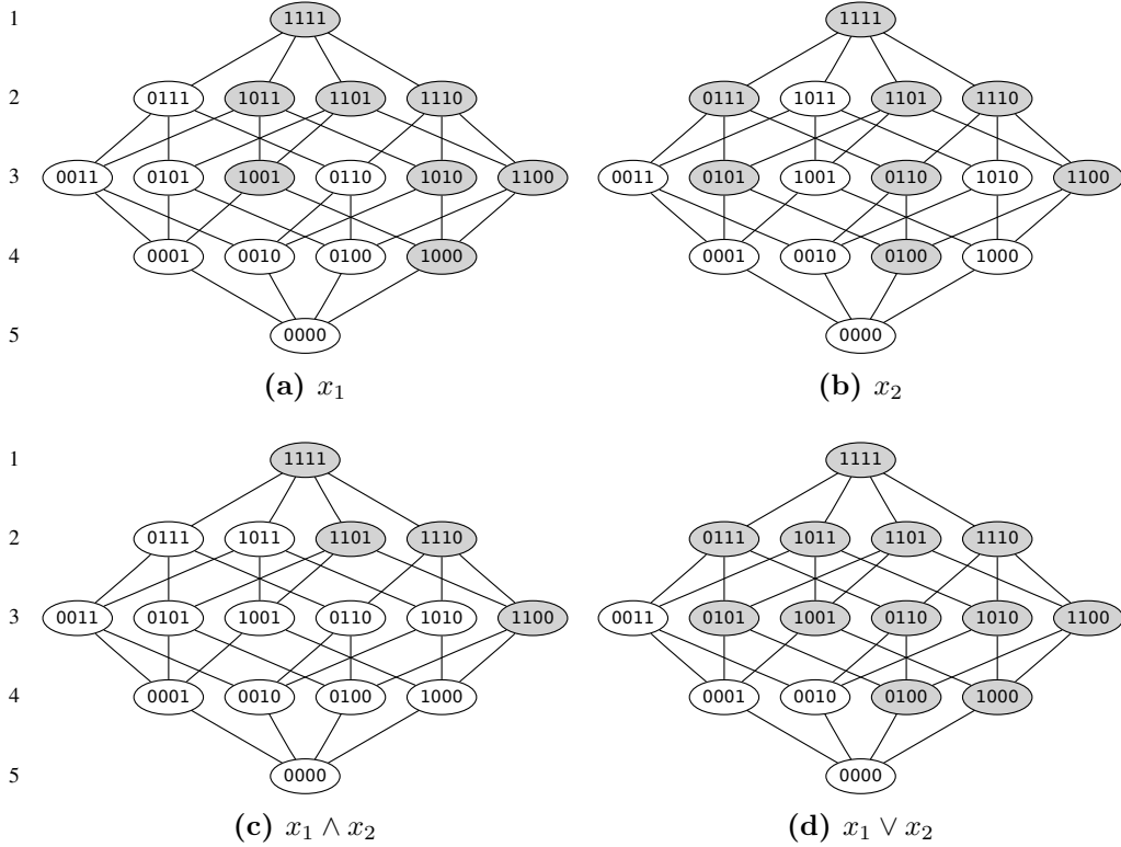
Figure 7: Comparator sharing to compute dual output functions in a 4-input sorting network. This figure illustrates the Boolean lattice representation of the functions computed by comparator 1 in Figure 6. The levels of the lattices are numbered on the left and the nodes at which the function takes the value 1 are shaded. Comparator 1 computes the conjunction (c) and the disjunction (d) of the functions (a) and (b) for the subgoal of computing the output functions f_1 = x_1 \wedge x_2 \wedge x_3 \wedge x_4 and f_4 = x_1 \vee x_2 \vee x_3 \vee x_4 . Function f_1 can be computed by utilizing conjunctions to set its value at all nodes in level 2 of the lattice to 0. Similarly, f_4 can be computed by utilizing disjunctions to set its value at all nodes in level 4 to 1. Thus, comparator 1 contributes to computing both f_1 and f_4 by setting the values at two nodes in level 2 of its conjunction to 0 and the values at two nodes in level 4 of its disjunction to 1. Sharing comparators in this manner reduces the number of comparators required to construct the sorting network.
