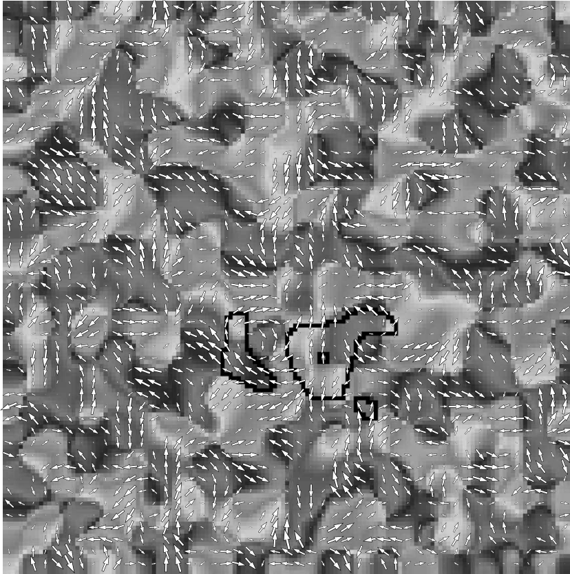
Fig. 3. Self-organized orientation and direction map. Through self-organization, a smoothly varying map of orientation and direction preferences emerged. Each of the 142 \times 142 neurons is colored with its preferred orientation, according to the key at right. The orientation map is similar to those found experimentally in animals, containing features such as pinwheels, linear zones, and fractures [13]. The direction preferences for every third neuron are plotted as white arrows overlaid on the orientation map. The size of each arrow is proportional to the neuron's directional selectivity, and the arrow points in the neuron's preferred motion direction. The preferred orientation is generally perpendicular to the preferred direction. As an example, the neuron from Fig. 2 is marked with a black square in the lower center of the plot. The neurons in that region of the map prefer horizontal stimuli moving upwards. Neurons in the patch just below the marked neuron also prefer nearly horizontal lines, but moving in the opposite direction. Other paired patches can be seen elsewhere in the map, as found experimentally [13]. The black outline shows the extent of the self-organized lateral weights for the marked neuron. The short-range connections target neurons with a variety of preferences, but long-range connections (a) target similar orientations and direction preferences, (b) extend along the orientation axis (horizontal), and (c) avoid orthogonal orientations and opposite directions. Animations of this plot are available at www.cs.utexas.edu/~nn .
