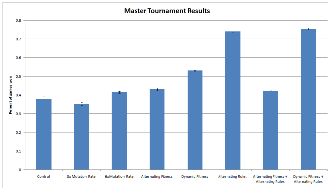
Fig. 3. Master Tournament Results. The percentage of games won by each method (i.e. the winners of 10 individual run tournaments of each method) averaged over five master tournaments. The actual numbers are shown in figure II. Alternating Rules, and especially when combined with Dynamic Fitness, results in significantly better performance than the other methods, although any form of shaping is better than none at all. The results thus demonstrate that shaping can be used to make coevolution more powerful.
