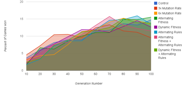
Fig. 4. Individual Run Tournament Results. Percentage of wins of each saved population in the 100-generation run is shown for each method. The curves generally trend up, suggesting that progress is made over evolution. However, there's significant difference in the win percentage of the first saved population (listed in detail in table III), suggesting that it can be used as an early check of whether the particular coevolutionary arms-race works well in the particular task.
