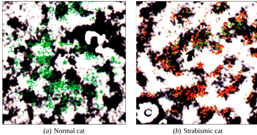
Fig. 5.2. Normal vs. strabismic cat ocular dominance maps and lateral connections. These plots show corresponding 5 mm \times 5 mm portions of the V1 ocular dominance maps from a normal cat (a) and from a cat raised with artificial strabismus (b). The maps were obtained using anatomical tracers, which result in categorical eye preferences (represented by light and dark areas instead of gray scale as in Figure 2.5). Both maps contain patches specific to each eye, but the patches are larger and more sharply delineated in the strabismic case. In (a), the green star indicates where fluorescent tracer was injected, and the green dots show where lateral retrograde transport took them. The lateral connection patterns do not significantly depend on the ocular dominance patterns. In (b), the red star and the green star (pointed by the arrow) mark two separate injection sites in right-eye columns (black). The lateral connections preferentially target neurons with the same eye preference (black patches, marked with red and green dots), and avoid neurons with the opposite eye preference (white). Each injection killed the nearby cells as a side effect, and therefore the ocular dominance and connection patterns are not visible in the areas surrounding the injections. Those areas are likely to be strongly connected to the neurons at the injection site. Detail of a figure by Löwel and Singer (1992), reprinted with permission, copyright 1992 by the American Association for the Advancement of Science.
