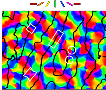
Fig. 5.3. Combined OR/OD map in the macaque. The orientation and ocular dominance maps shown separately in Figure 2.5 are overlaid in this plot. Color encodes OR preference (according to the key on top; example map features are outlined in white as in Figure 2.4), and the black outlines represent OD stripe boundaries, obtained as areas of high OD gradient. The features in the two maps are systematically organized. The OD boundaries intersect the OR boundaries of linear zones (long rectangle) at right angles, and rarely follow an OR boundary. Pinwheel centers (circles) are usually found well inside the OD stripes, and rarely near their boundaries. Note that, unlike the small patches seen in the cat OD maps (Figure 5.2), the OD patches in the monkey typically consist of long stripes (as also shown in Figure 2.5b). Reprinted with permission from Blasdel (1992b), copyright 1992 by the Society for Neuroscience; annotations added, OD contours replotted from data by Blasdel (1992a).
