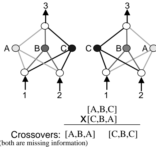
Figure 1: The competing conventions problem. The two networks compute the same exact function even though their hidden units appear in a different order and are represented by different chromosomes, making them incompatible for crossover. The figure shows that the two single-point recombinations are both missing one of the 3 main components of each solution. The depicted networks are only 2 of the 6 possible permutations of hidden unit orderings.
