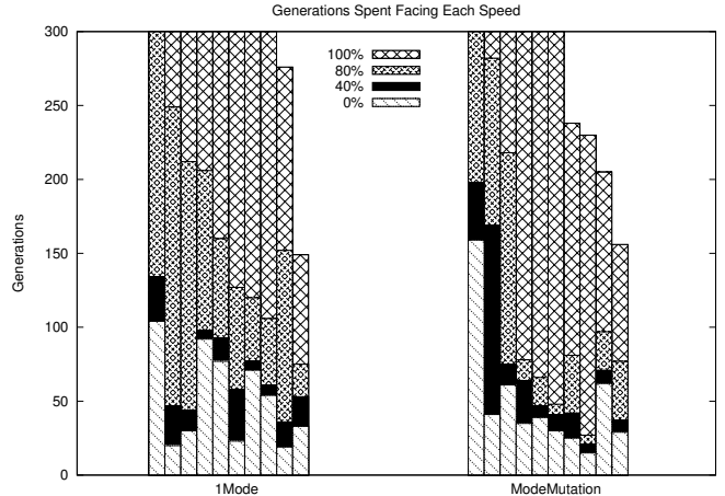
Fig. 4. Generations Spent Facing the Bot at Each Speed: For the ten 1Mode trials and ten ModeMutation trials, the generations spent facing the bot at 0%, 40%, 80% and 100% speed are shown in a stacked bar chart. Four ModeMutation trials and two 1Mode trials finished before reaching the 300 generation cutoff.
