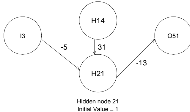
Figure 3: An example node definition in a marker-based gene. For example, the first connection has key = 82 , label = 3 , w = -5 . The key and label are both positive so the connection is to be made from input unit 3. The last connection wraps around to the beginning of the chromosome.
