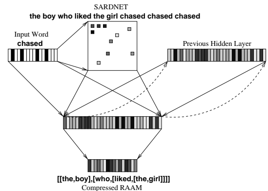
Figure 2: The SARDSRN Network. This snapshot shows the network during step 11 of figure 1. The representation for the current input word, chased , is shown at top left. Each word is input to the SARDNET map, which builds a representation for the sequence word by word. At each step, the previous activation of the hidden layer is copied (as indicated by the dotted line) to the Previous Hidden Layer assembly. This activation, together with the current input word and the current SARDNET pattern, is propagated to the hidden layer of the SRN network. As output, the network generates the compressed RAAM representation of the top element in the shift-reduce stack at this state of the parse (in this case, line 12 in figure 1). SARDNET is a map of word representations, and is trained through the Self-Organizing Map (SOM) algorithm [Kohonen, 1995; 1990]. All other connections are trained through backpropagation.
