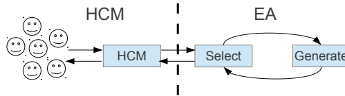
Fig. 2: The IEC+HCM approach. During each generation of evolution, when evaluating the population the EA uploads evaluation tasks to the HCM to be completed by human users. The results guide which parents reproduce to form the next generation. In this way, an EA can be driven by the human judgment of many non-experts.
