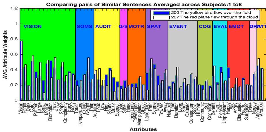
Figure 3: Contrasting the conceptual combination effect in two different sentences. In Sentence 200 (blue bars), the CAR representation modified by FGREP for the word flew has salient activations on animate features, likely denoting bird properties like Pain, Smell and Taste, and Communication. In Sentence 207 (white bars), it has high activations on inanimate object features, describing a Loud, Large, and Heavy object such as a plane . Thus, there is a clear difference between animate and inanimate features found in each sentence.
